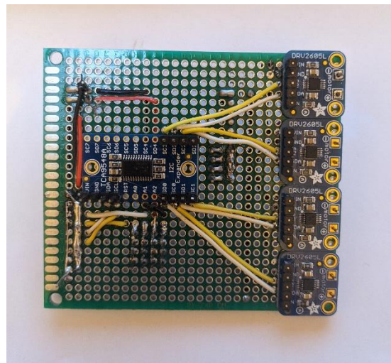
Figure 2.4: Top view of the circuit board which contains the haptic drivers (right side) and I2C Multiplexer (centre).
